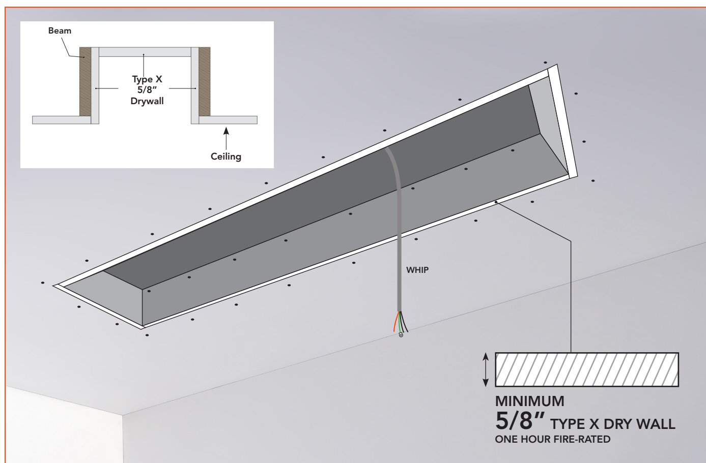
61" FLUSH MOUNT FRAME
