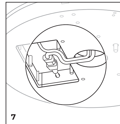
Connect the LED and power cables in the base of the unit.
