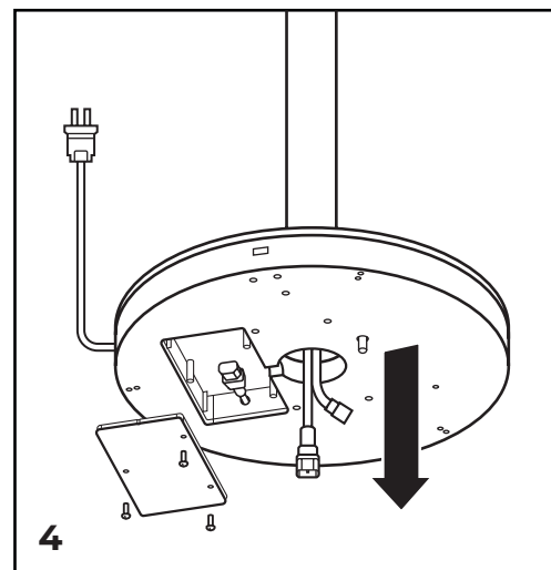
Feed the power cords from the unit assembly through the base of the pole.
