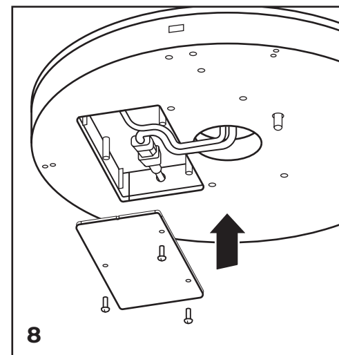
Re-install the wiring compartment cover.
